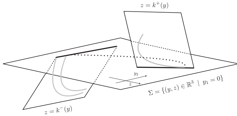
Fig. 5. DDAE. The dotted curve is the set G(y, z) = 0 . The lighter curves are solution trajectories in R^- and R^+ .
