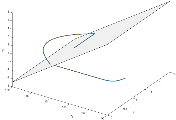
Fig. 10. Numerical solutions of the Singularly Perturbed system and of the Direct Approach system.
