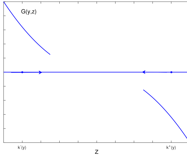
Fig. 3. Plot of the function G = G(y, z) for y fixed in function of z .
