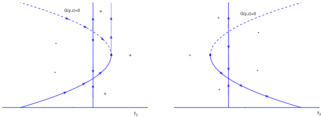
Fig. 4. Theorem 13. Case (ii)_1 in left plot and Case (ii)_2 in the right plot.
