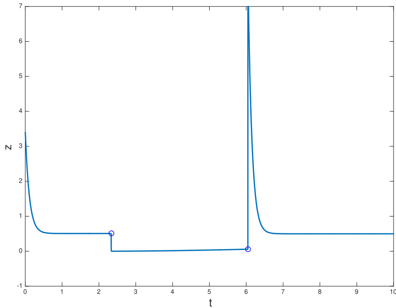
Fig. 11. Numerical approximation of the algebraic variable computed with the Singular Perturbation Approach.
