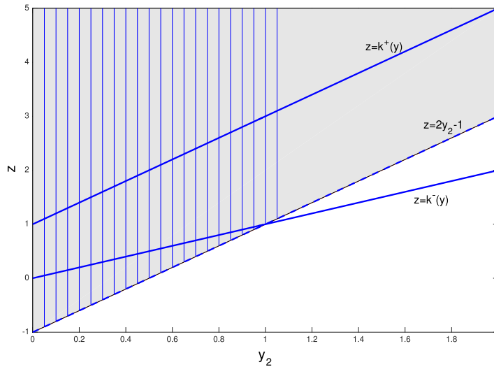
Fig. 6. Example 17. Attractive region for (41) (the shaded area) and set \Sigma_K (the striped area).
