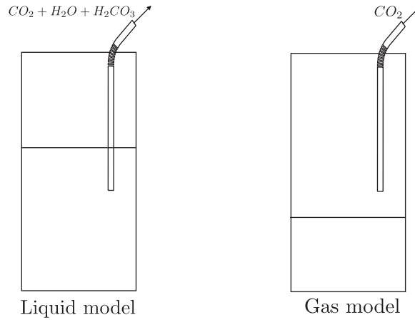
Fig. 9. Ideal gas liquid model.
