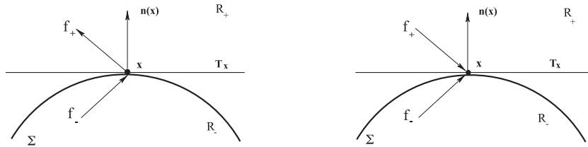
Fig. 1. Crossing and sliding point.
